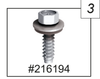
Gewindeschneidschraube JZ3-6,3x38 Thread cutting screw JZ3-6,3x38
